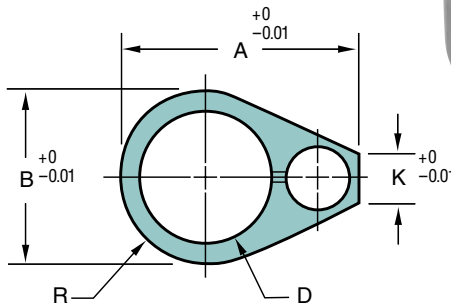
Ball hole location radial tolerance \pm 0^{\circ}5'
