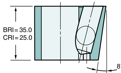
Ball hole location radial tolerance \pm 0^{\circ}5'
